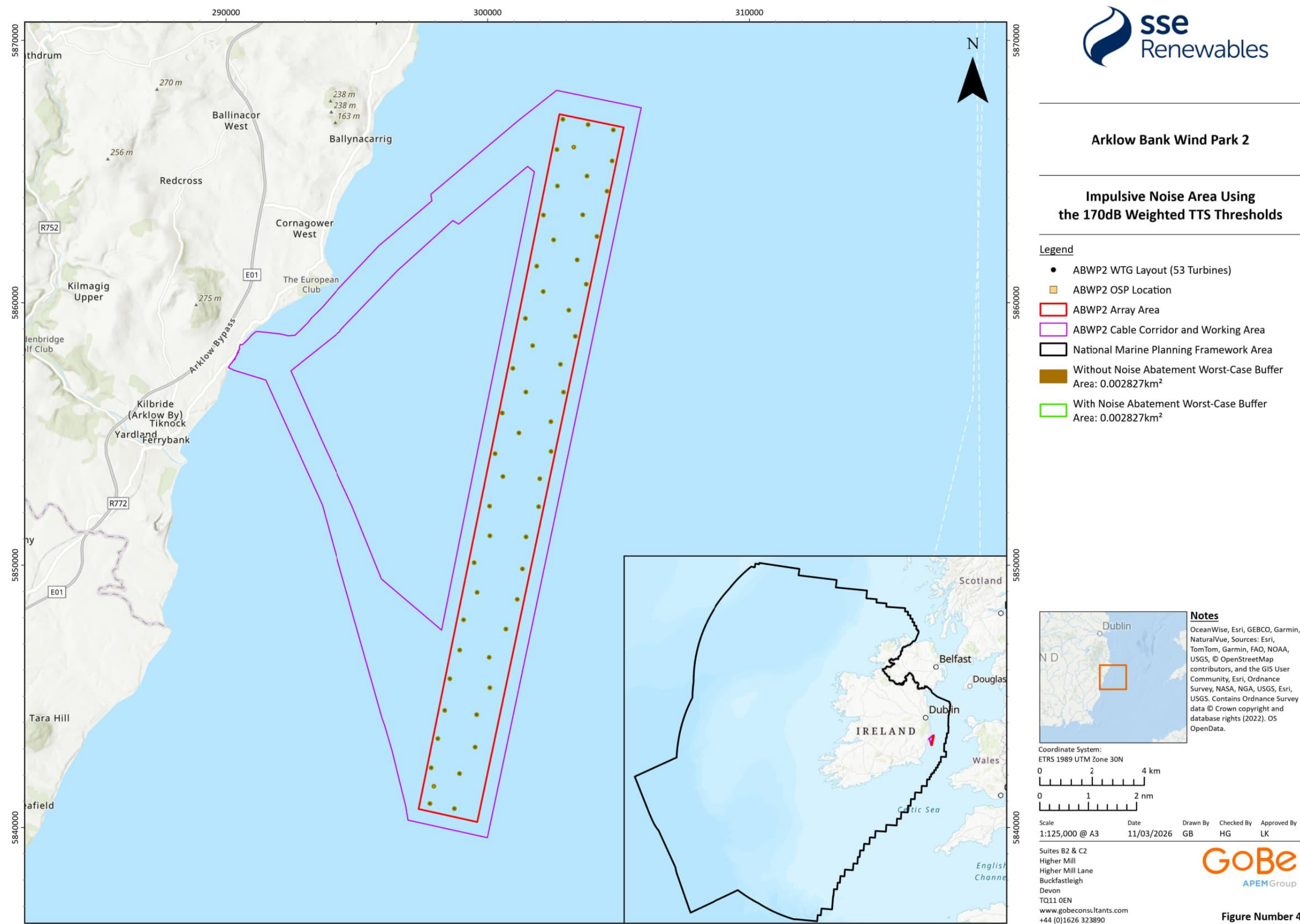
Figure 4 Impulsive Noise Area Using the 170dB Weighted TTS Threshold for with and without noise abatement scenarios
