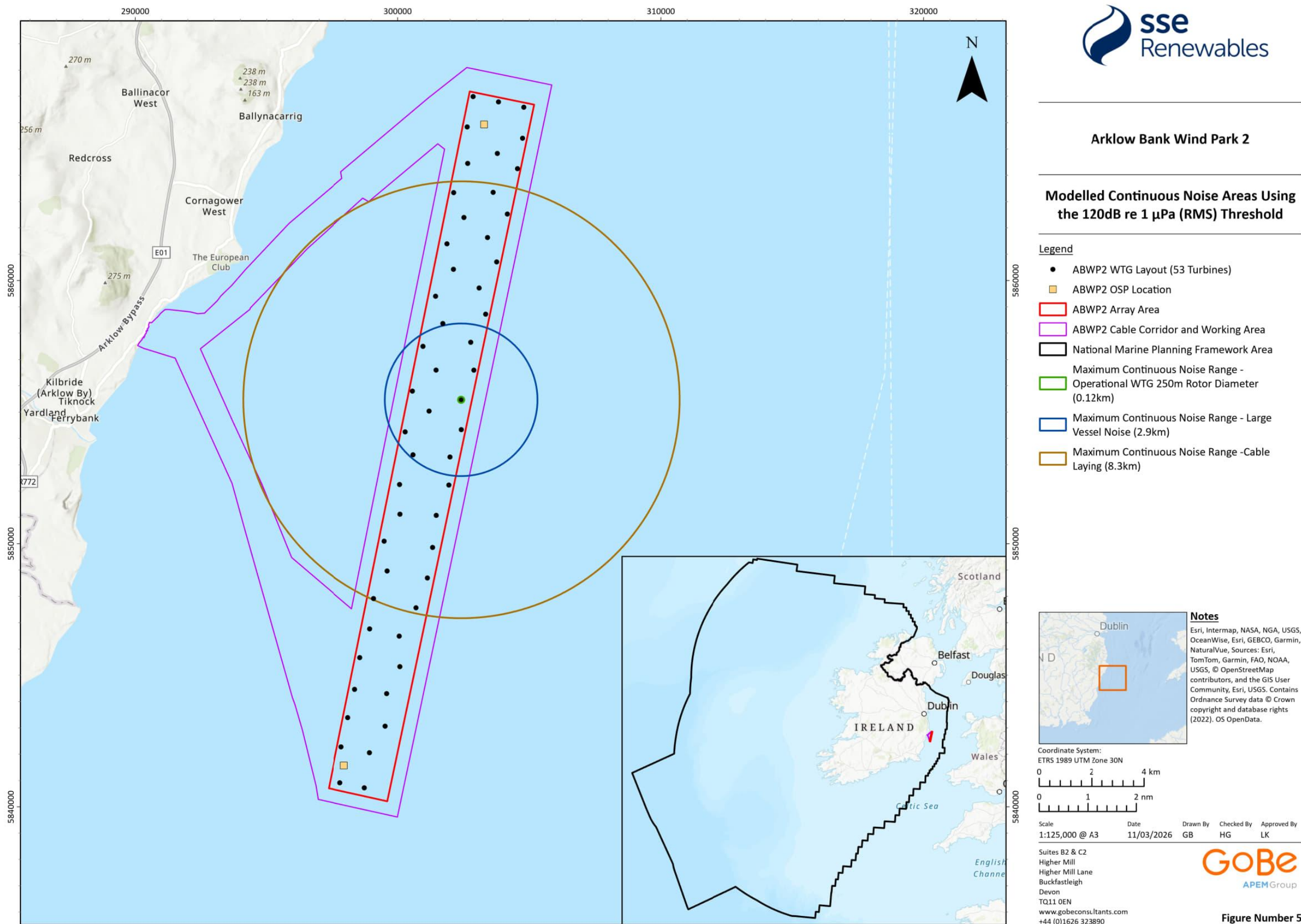
Figure 5 Modelled Continuous Noise Areas using the 120 dB re 1 \mu Pa (RMS) Threshold
